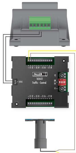
Fig. 7: Connection diagram Branch-off junction / Traffic Control
