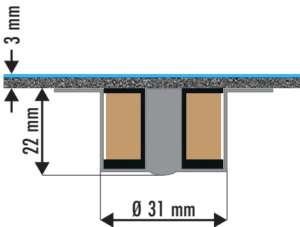
Fig. 10: Stop section, Cross section
