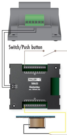
Fig. 13: Connection diagram Stop section, manual operation
