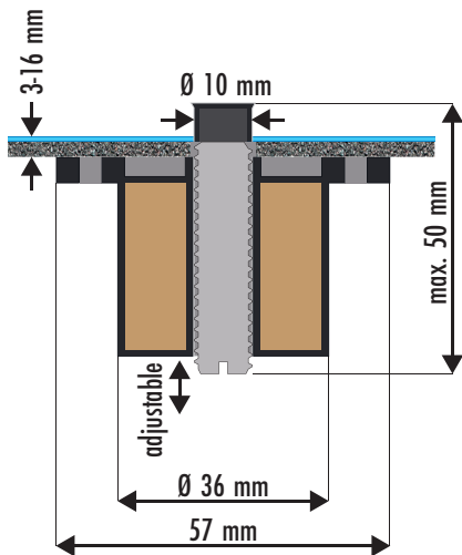
Fig. 18: Parking space, Cross section, elevated spacer
