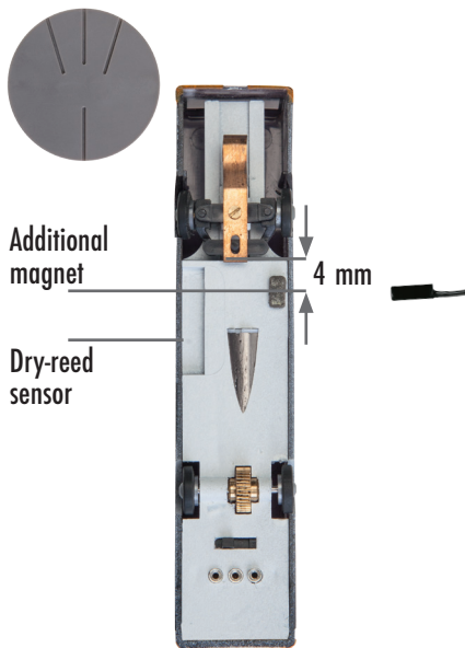
Fig. 25: Additional magnet N
