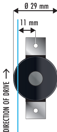
Fig. 9: Stop section with contact wire, Top view
